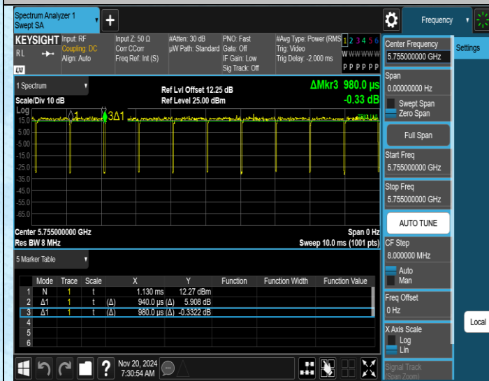
NTNV-11N40SISO-Ant1-5755
