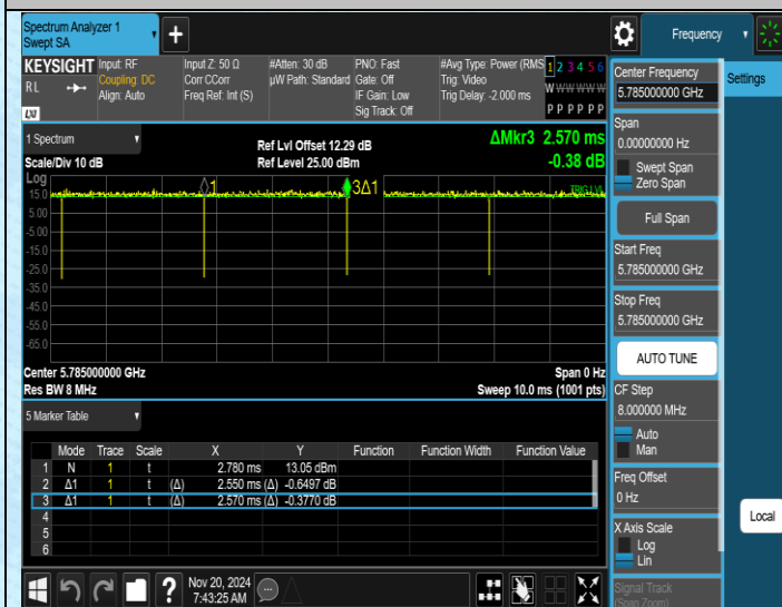
NTNV-11AC20SISO-Ant1-5785
