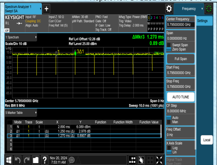
NTNV-11AC40SISO-Ant1-5795
