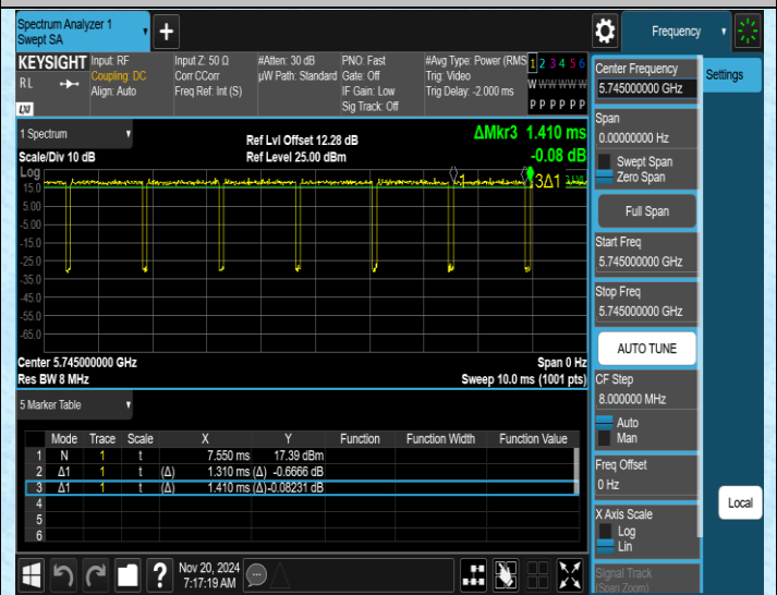
NTNV-11N20SISO-Ant1-5745
