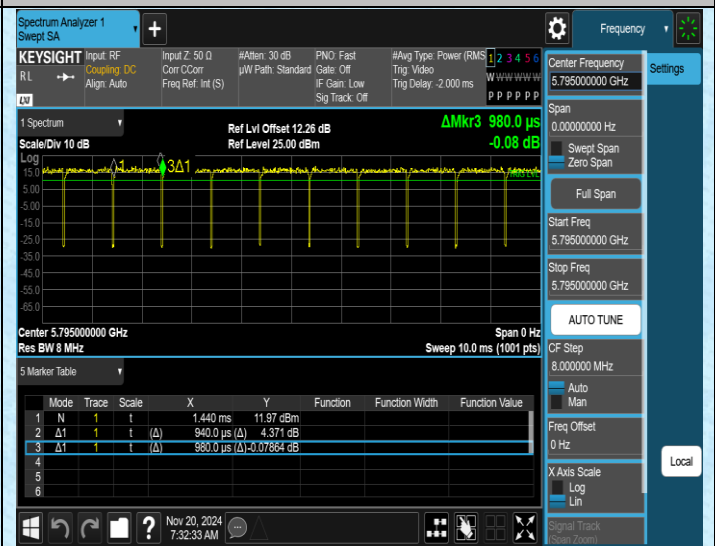
NTNV-11N40SISO-Ant1-5795
