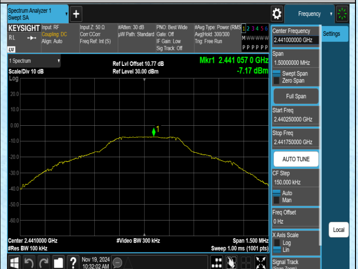
DH5-Ant1-2441-0-Reference-PASS
