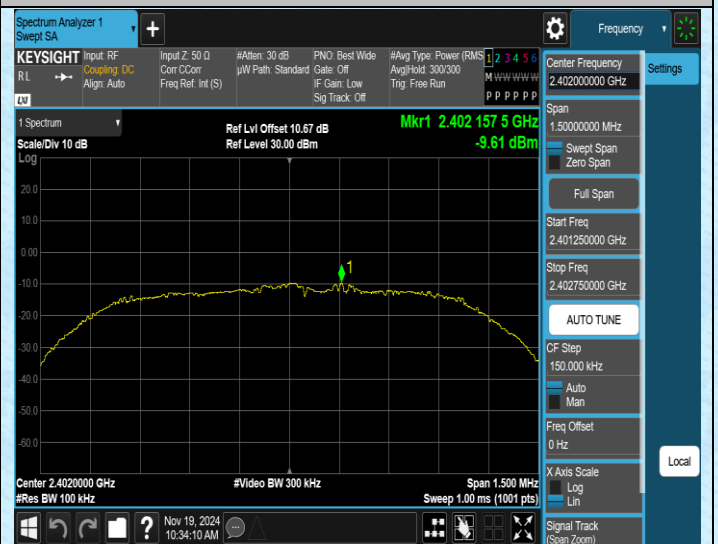
2DH5-Ant1-2402-0-Reference-PASS
