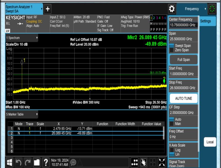
2DH5-Ant1-2480-1000-26500-PASS
