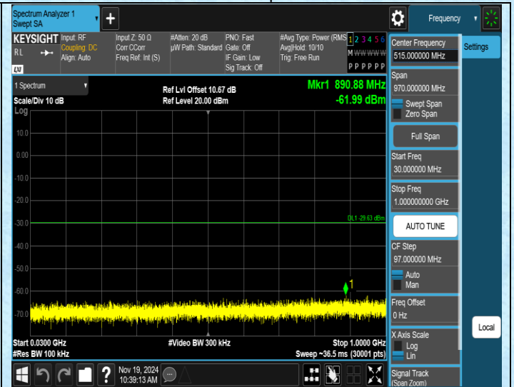
3DH5-Ant1-2402-30-1000-PASS
