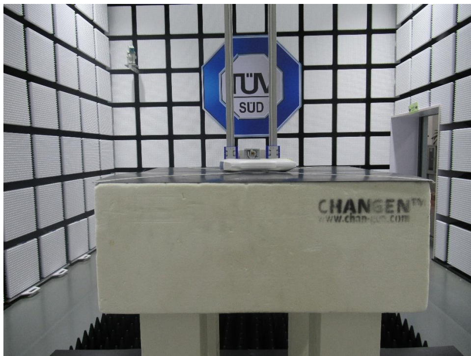
Spurious emission test above 18GHz
