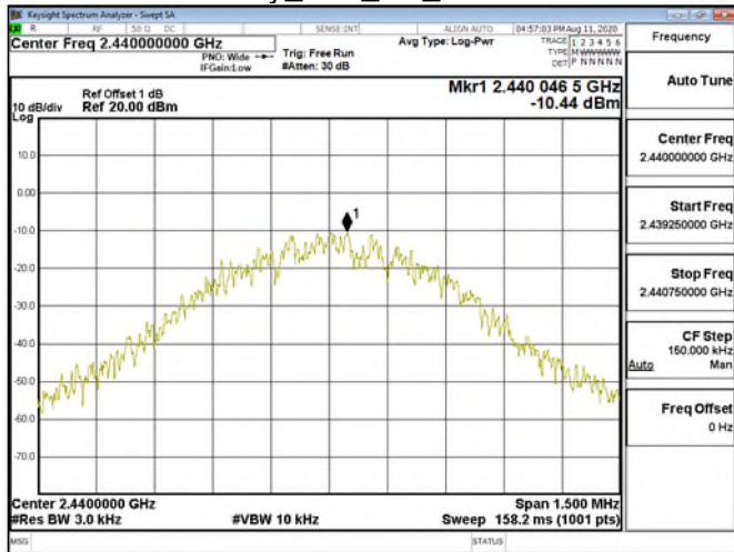
Power Density_BLE_1M_LowCH19-2440
