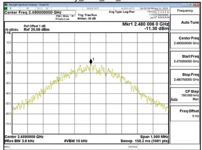
Power Density_BLE_1M_LowCH39-2480
