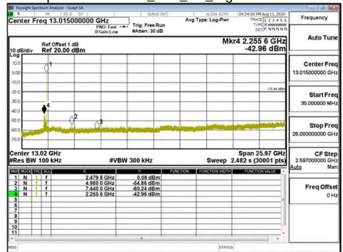
Spurious Emission_BLE_1M_HighCH39-2480
