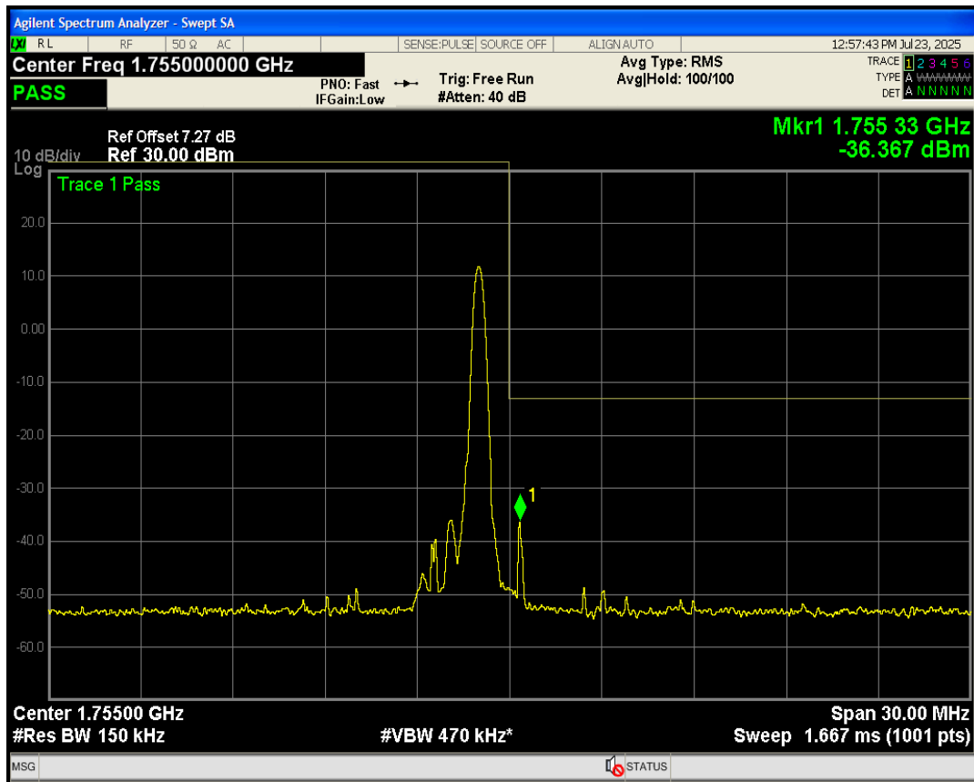
Band4 QAM16 BW=15MHz Channel=20325 RB Size=6 Position=#Max NB Index=1
