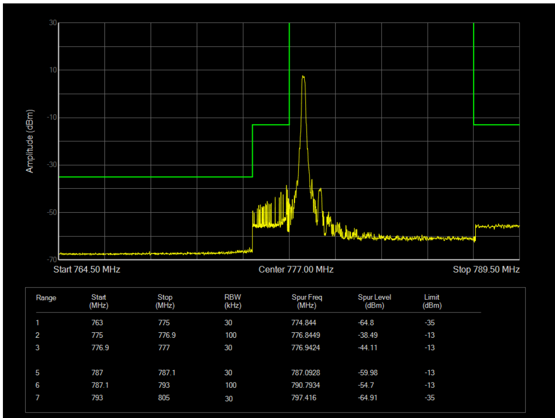
Band13 QAM16 BW=10MHz Channel=23230 RB Size=4 Position=#0 NB Index=0
