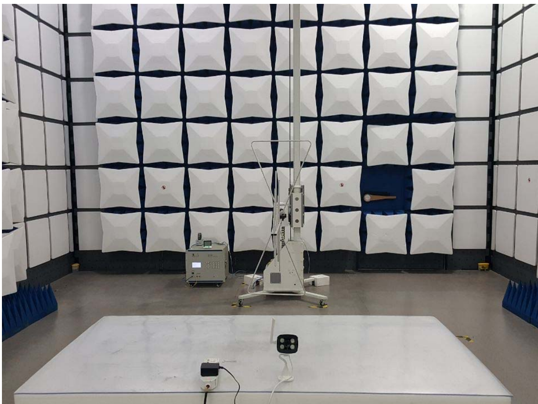
Radiated Emissions
