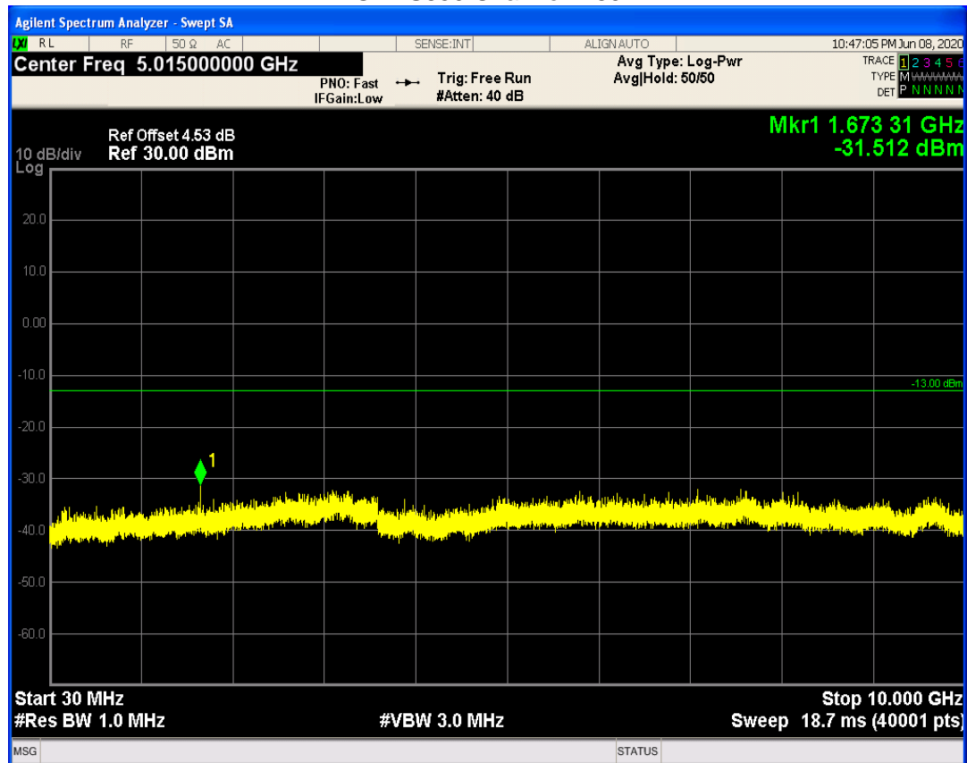
GPRS850 Channel=189
