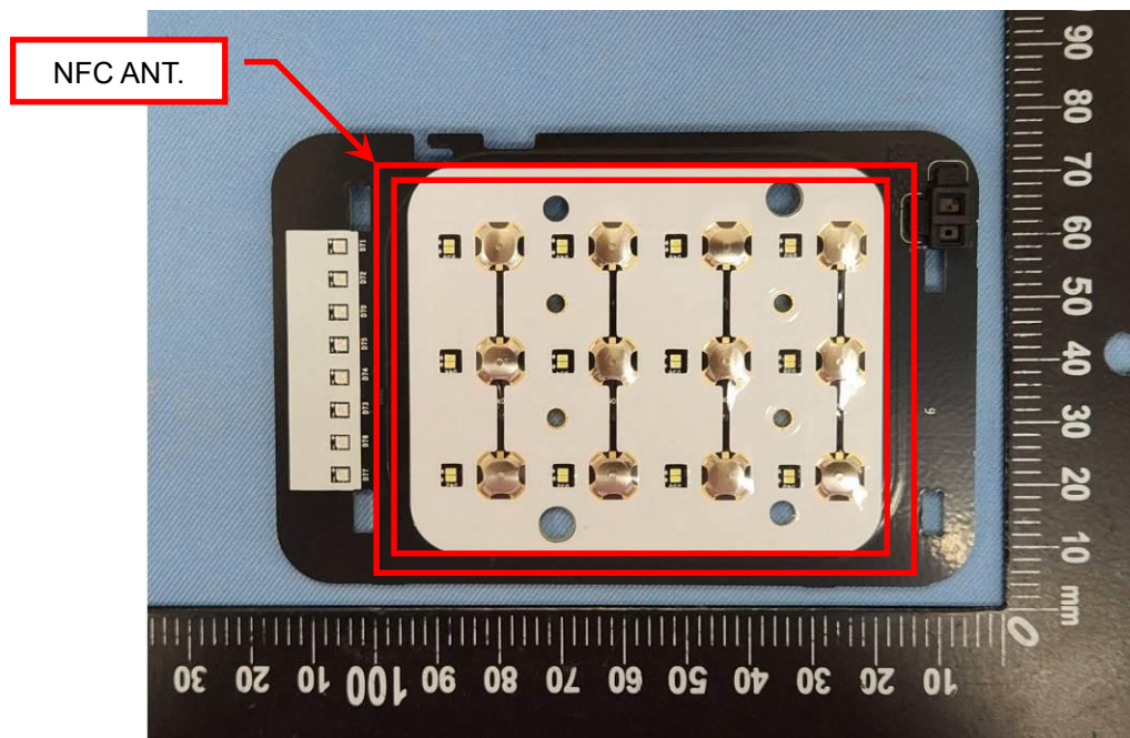
EUT Photo (22)
