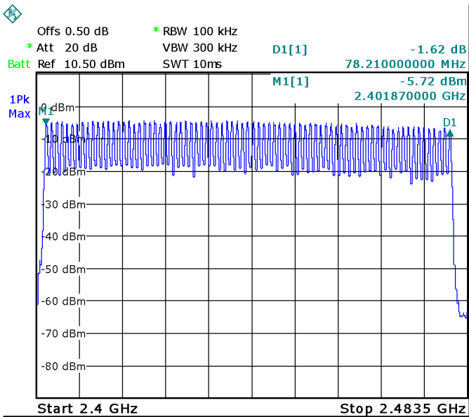
Modulation: GFSK
