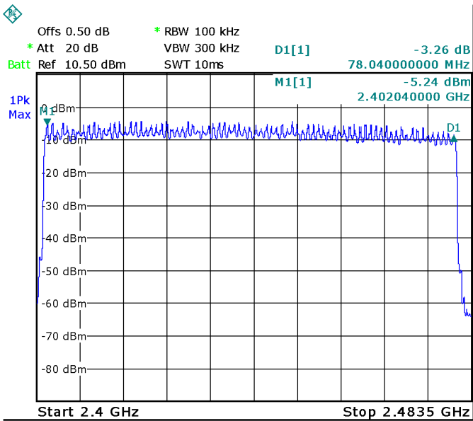
Modulation: 8DPSK
