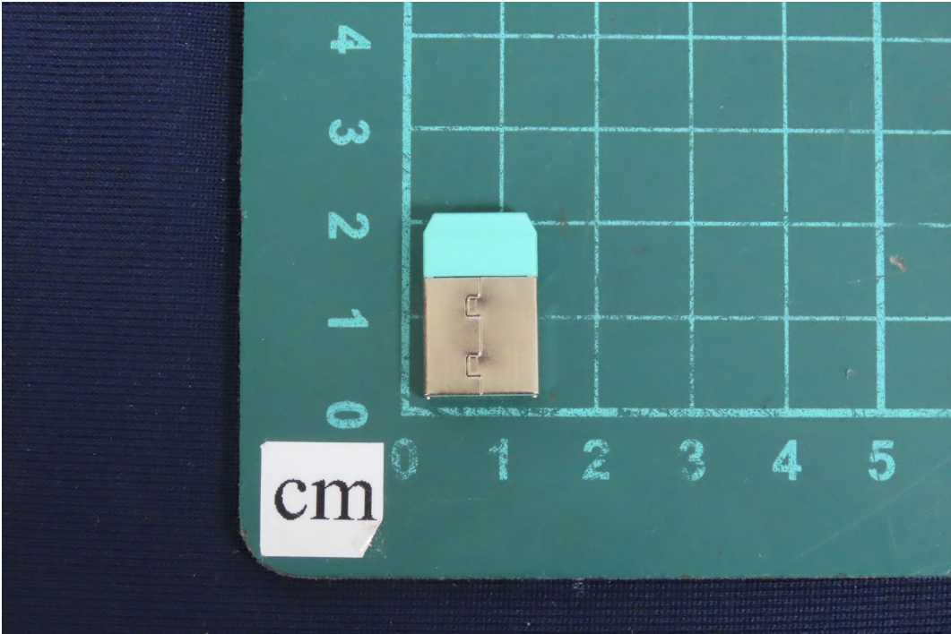
(21) EUT PhotoDongle
