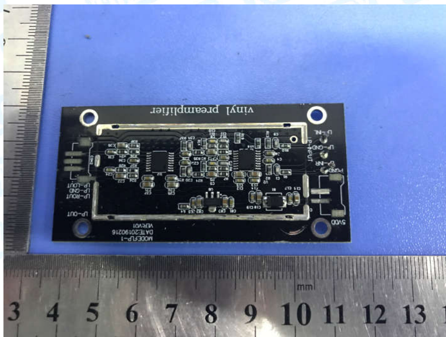
Photo 23 Internal of PCB
