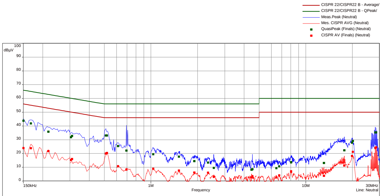
CISPR 22/CISPR22B
