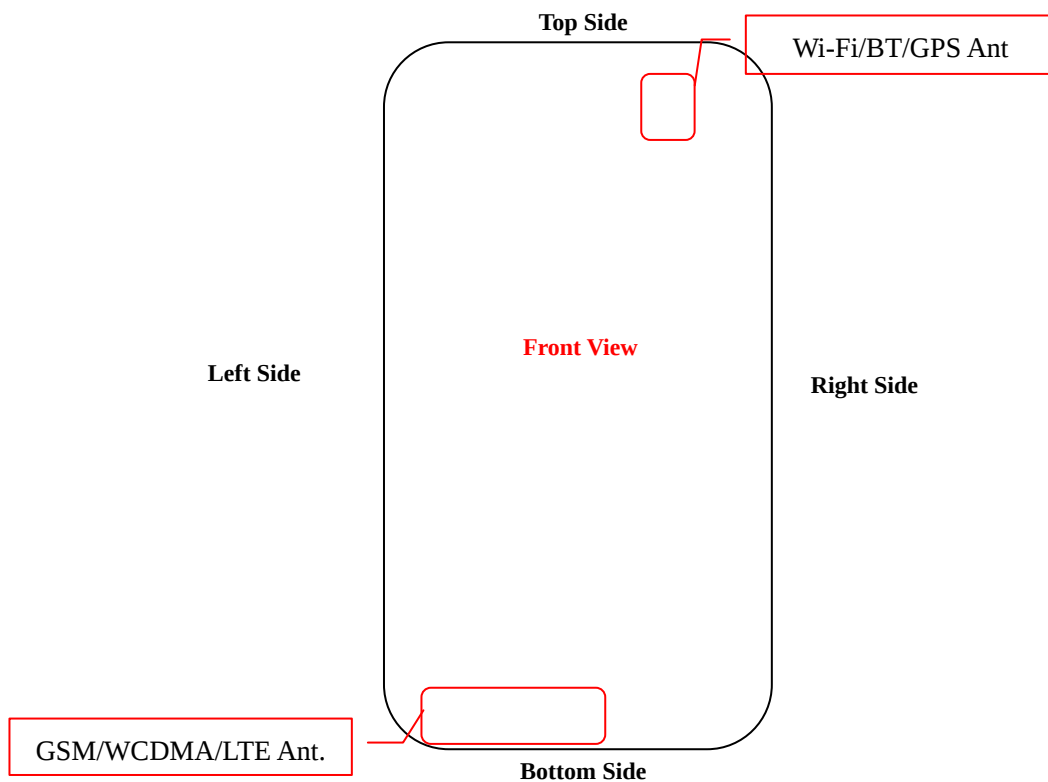
Block Diagram for EUT Antenna Position
