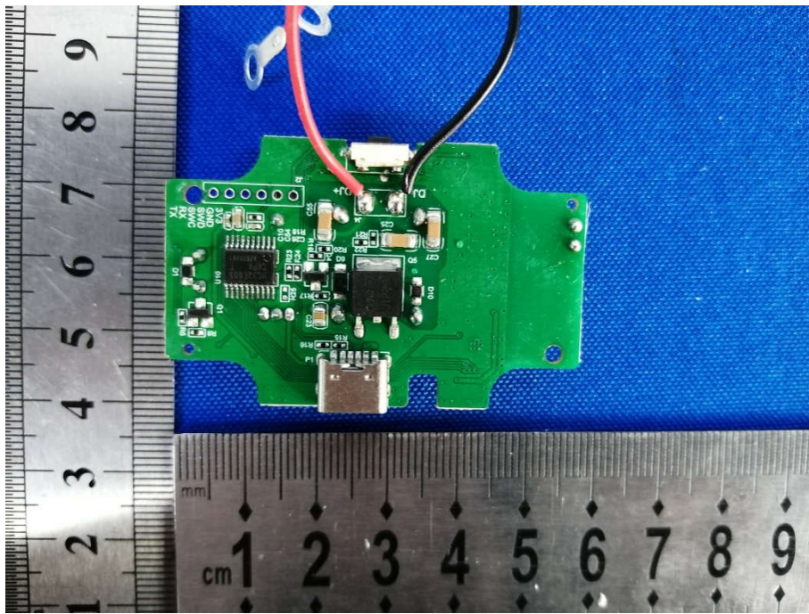
View of PCB Layout of AFU-WOH-0002B
