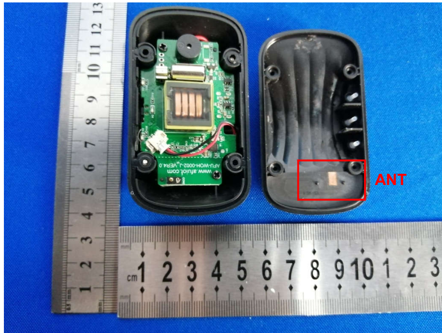
Internal view of AFU-WOH-0002B
