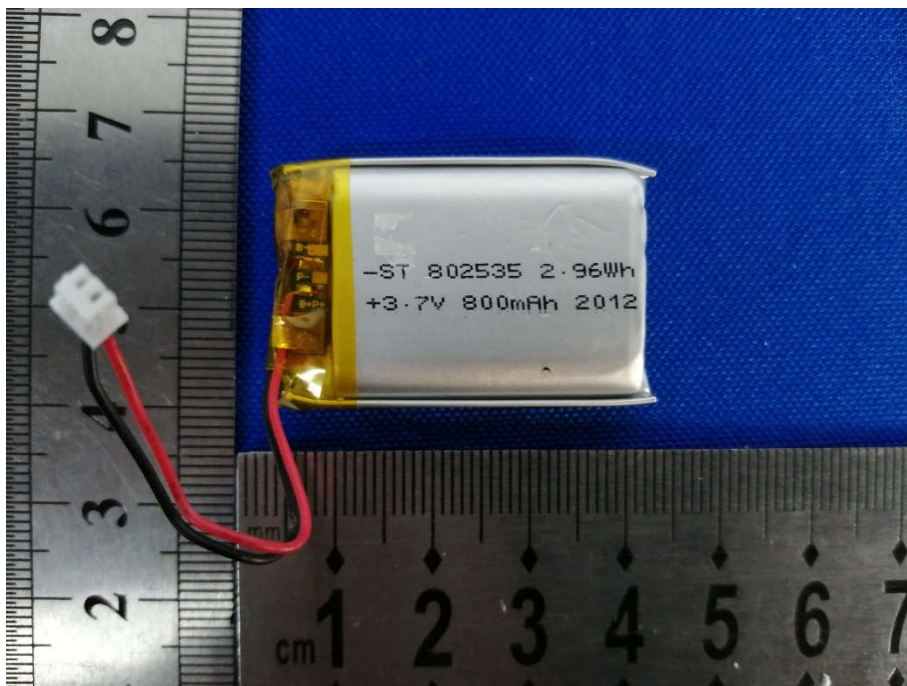
View of Li-ion of AFU-WOH-0002B
