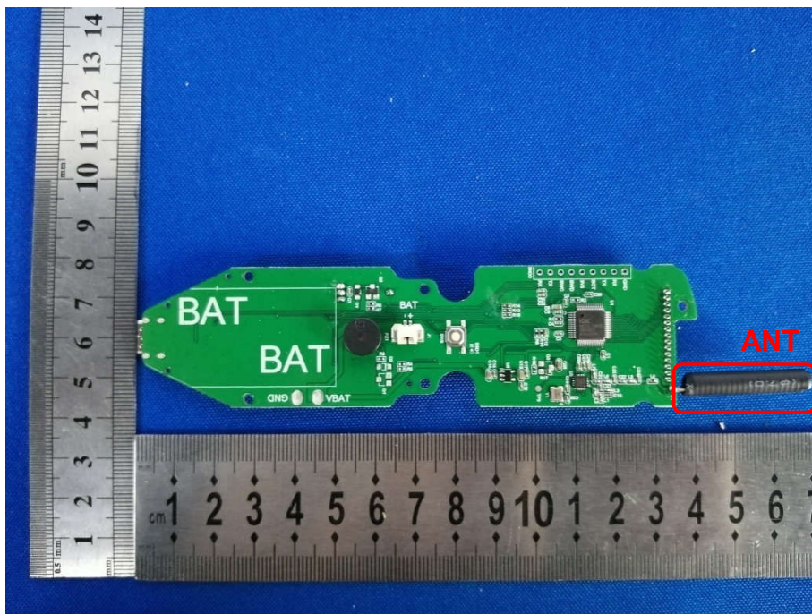
View of PCB Layout of AFU-WOH-0002A
