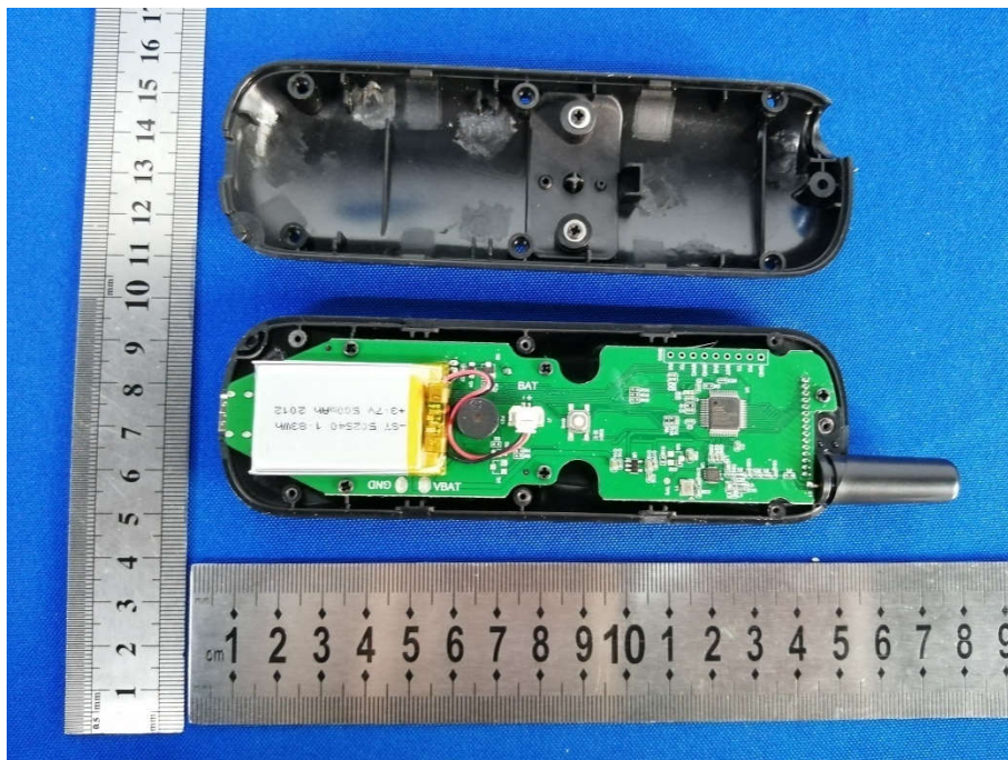
Internal view of AFU-WOH-0002A
