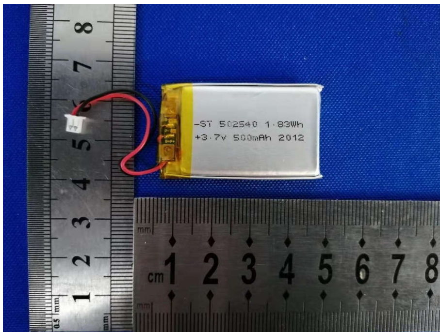
View of Li-ion of AFU-WOH-0002A
