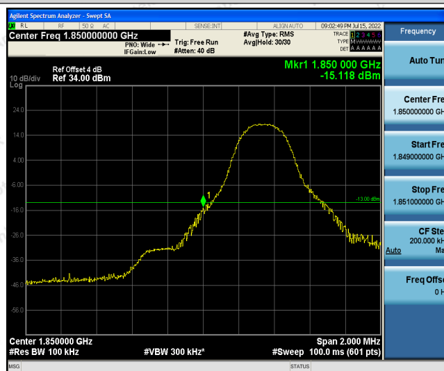
Band25-5MHz-QPSK-26065-1RB#24
