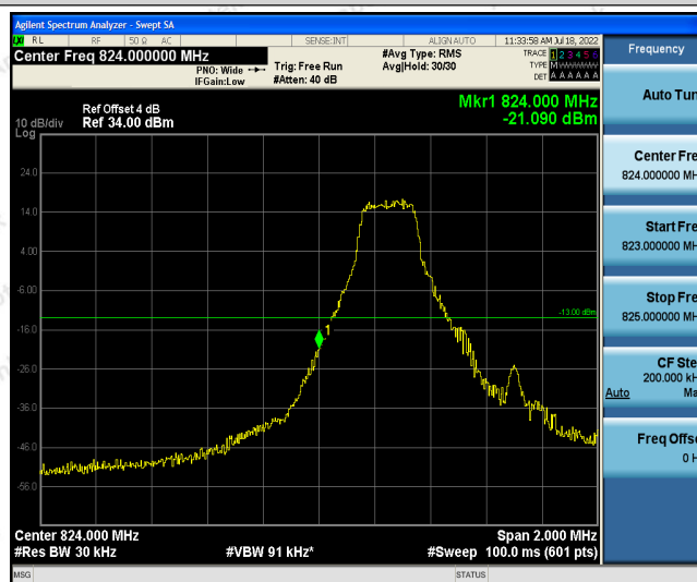
Band26-1.4MHz-16QAM-26797-1RB#5
