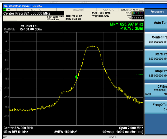
Band26-3MHz-QPSK-26805-1RB#14
