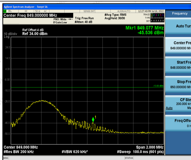
Band26-10MHz-16QAM-26990-1RB#49
