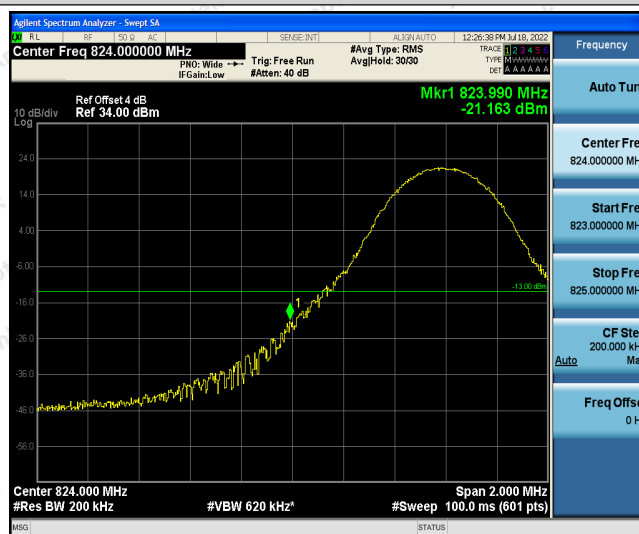
Band26-10MHz-16QAM-26840-1RB#49
