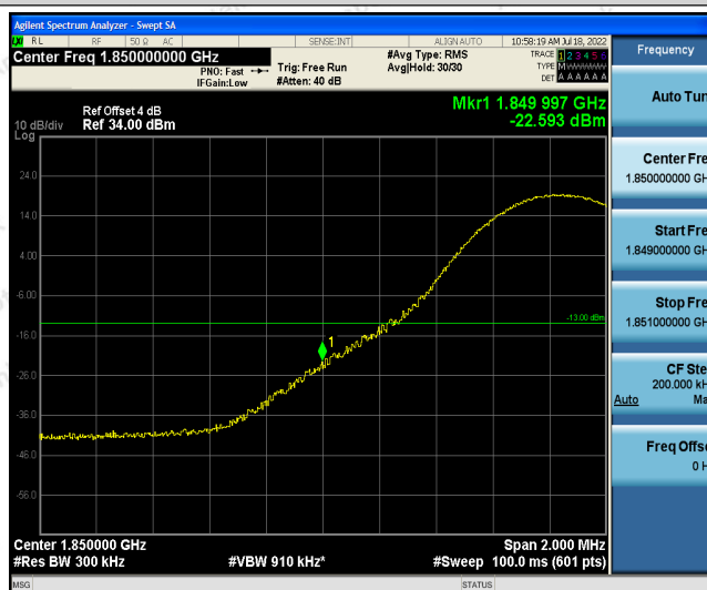
Band25-15MHz-16QAM-26115-1RB#74
