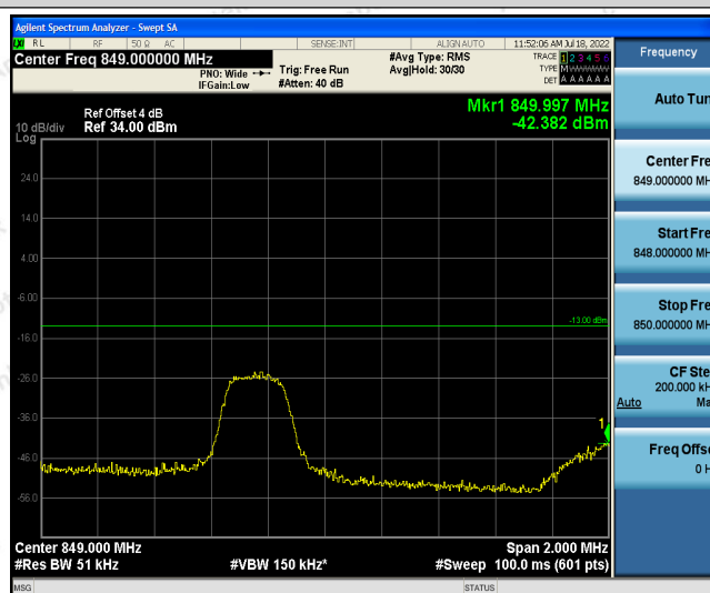
Band26-3MHz-16QAM-27025-1RB#14
