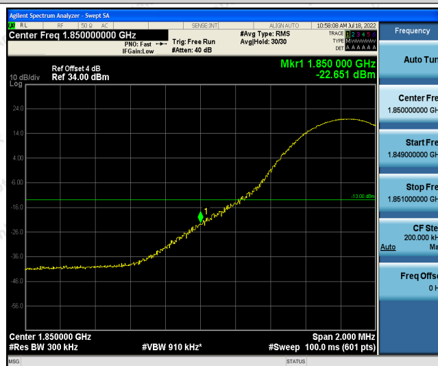
Band25-15MHz-QPSK-26115-1RB#74
