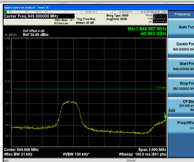
Band26-3MHz-QPSK-27025-1RB#14
