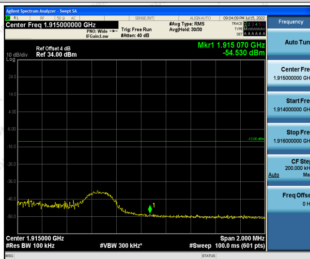
Band25-5MHz-16QAM-26665-1RB#24
