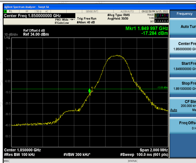
Band25-5MHz-16QAM-26065-1RB#24
