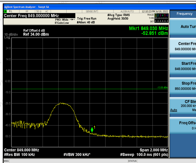
Band26-5MHz-16QAM-27015-1RB#24
