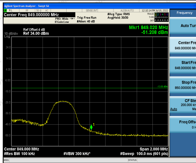
Band26-5MHz-QPSK-27015-1RB#24
