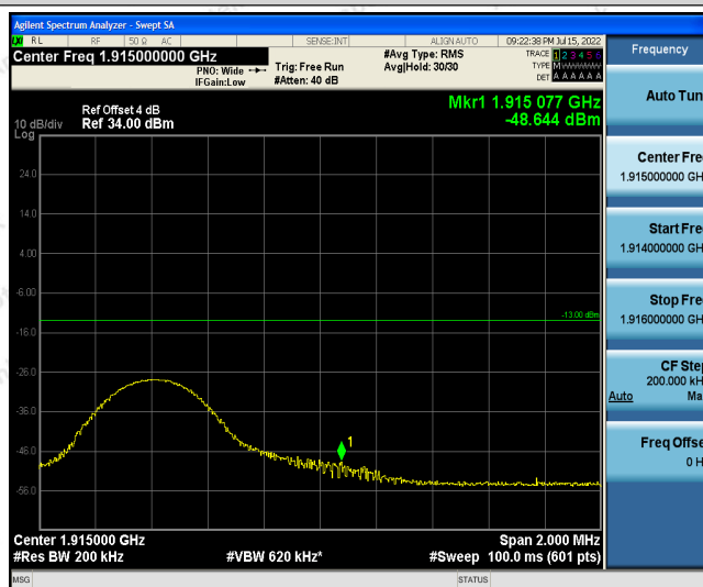
Band25-10MHz-QPSK-26640-1RB#49
