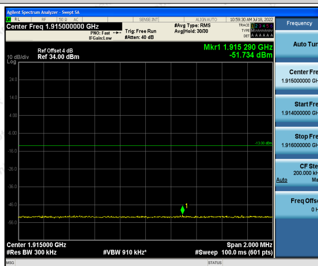
Band25-15MHz-16QAM-26615-1RB#74
