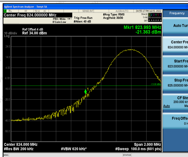
Band5-10MHz-16QAM-20450-1RB#49
