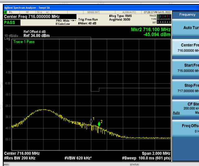
Band12-10MHz-16QAM-23130-1RB#49
