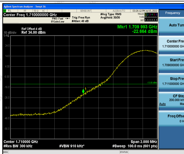
Band4-15MHz-16QAM-20025-1RB#74
