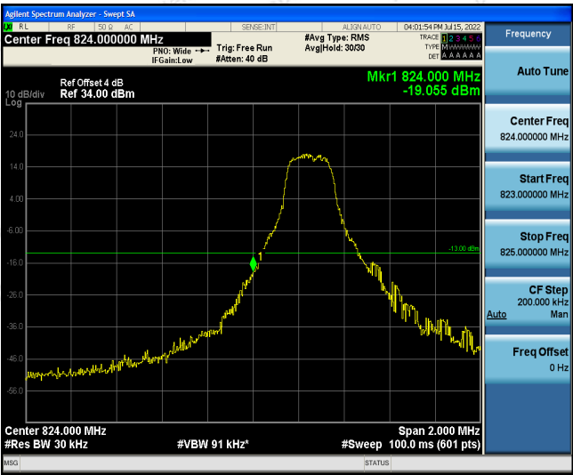
Band5-1.4MHz-QPSK-20407-1RB#5
