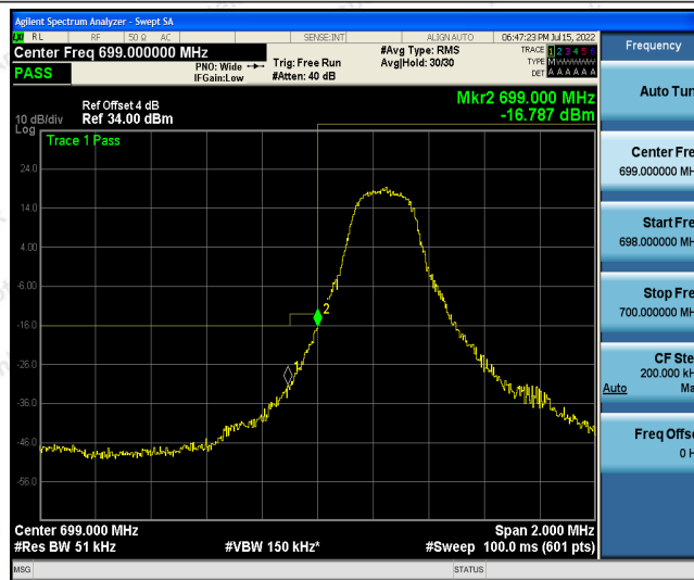
Band12-3MHz-QPSK-23025-1RB#14
