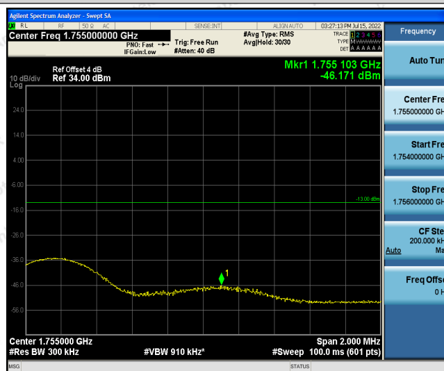
Band4-15MHz-QPSK-20325-1RB#74
