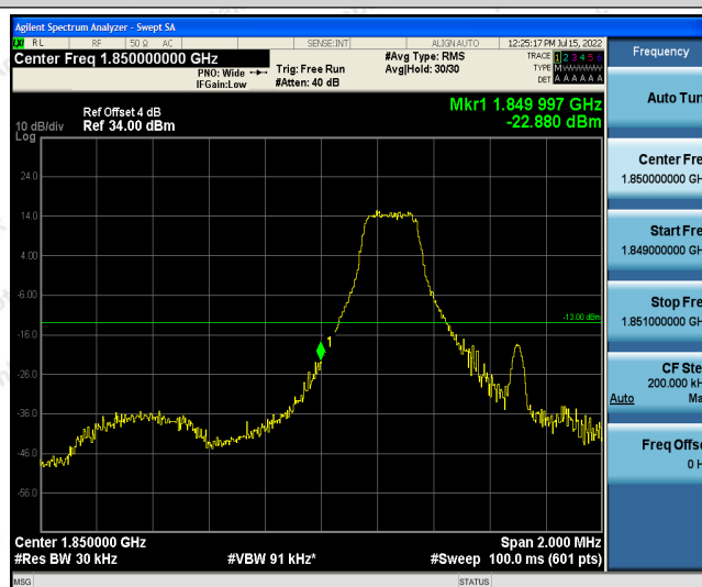
Band2-1.4MHz-16QAM-18607-1RB#5
