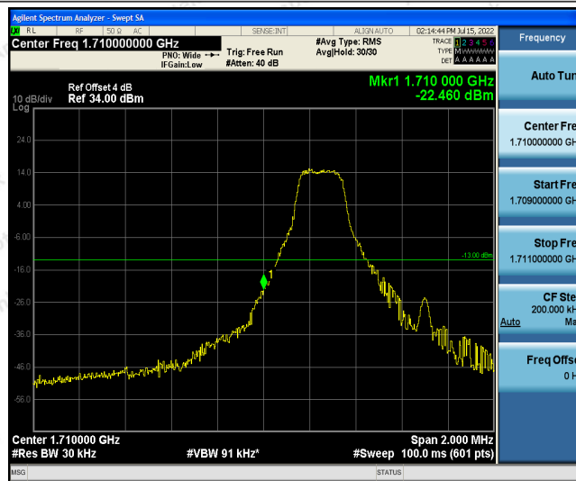
Band4-1.4MHz-16QAM-19957-1RB#5
