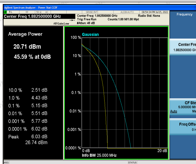
Band25-3MHz-QPSK-26675-1RB#0
