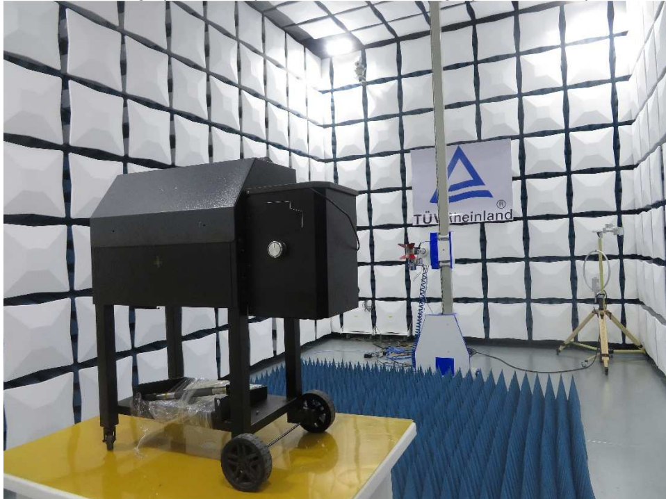
Photograph 1: Set-up for Radiated band edge (1GHz-18GHz)
