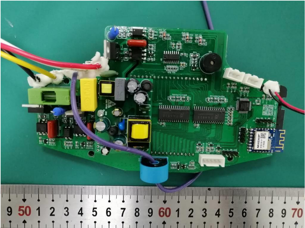
PCBs of the EUT
