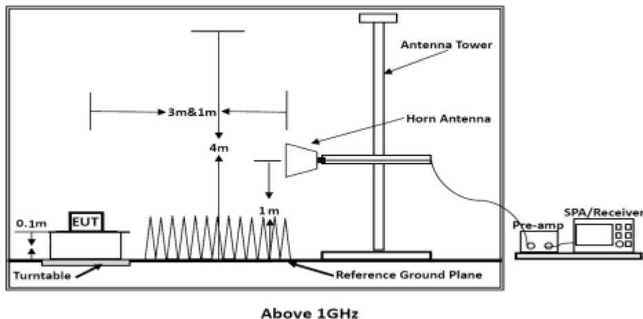
Figure 3. Above 1GHz
