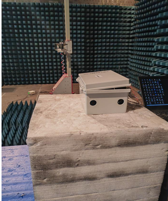
RE above 1GHz
