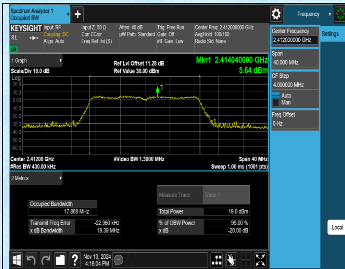
11N20SISO-Ant1-2412
