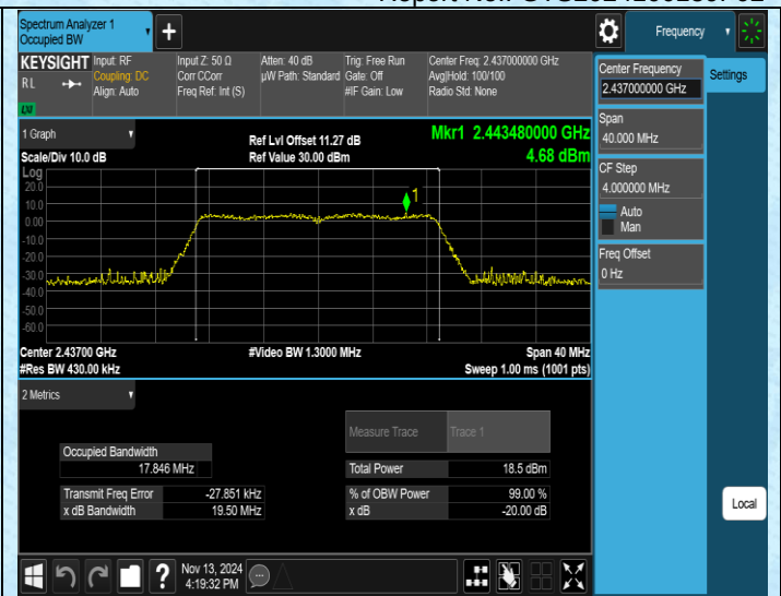
11N20SISO-Ant1-2437
