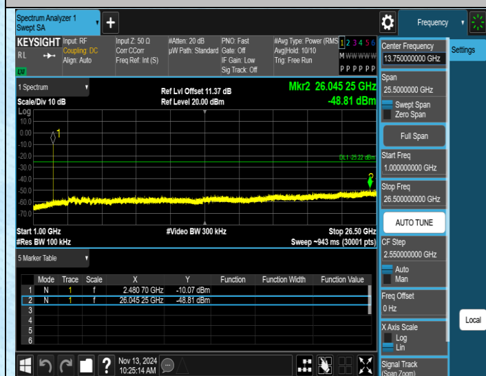
3DH5-Ant1-2480-1000~26500-PASS
