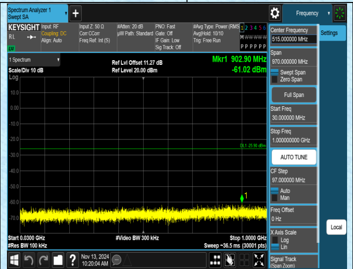
2DH5-Ant1-2441-30~1000-PASS
