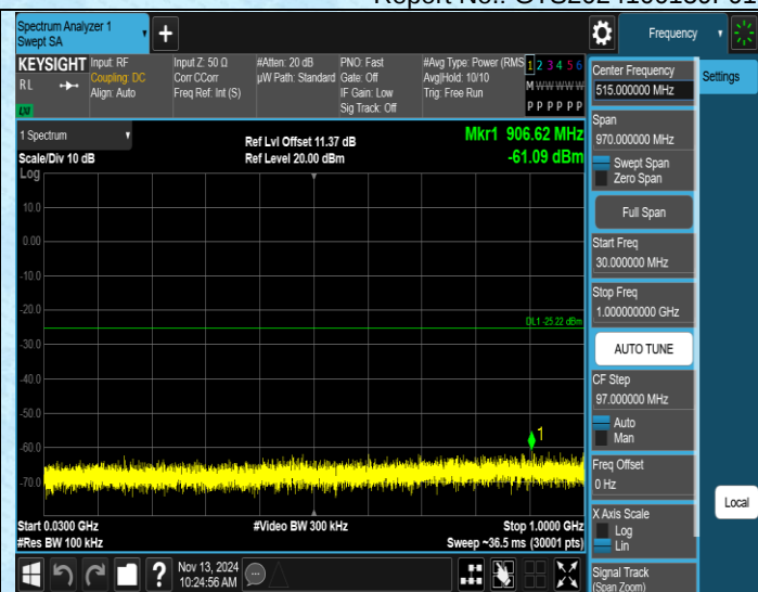
3DH5-Ant1-2480-30~1000-PASS
