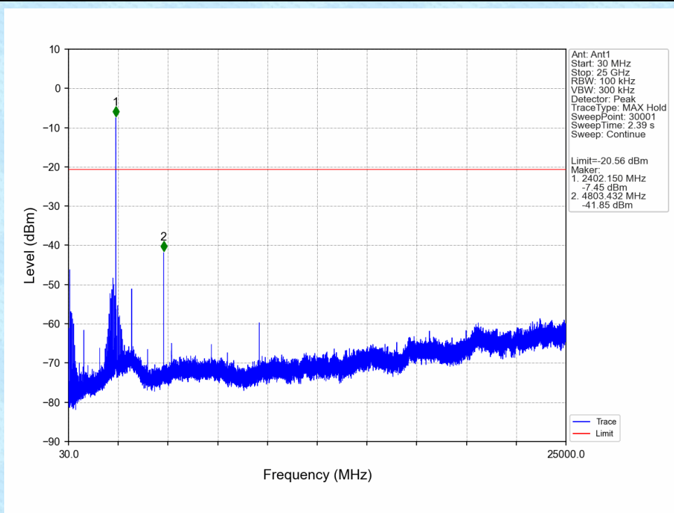
8DPSK_3DH5_LCH_2402MHz_Ant1_NTNV
