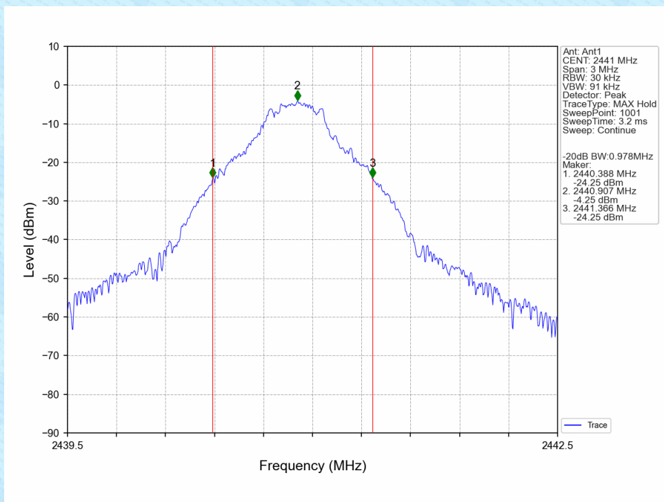
GFSK_DH5_MCH_2441MHz_Ant1_NTNV
