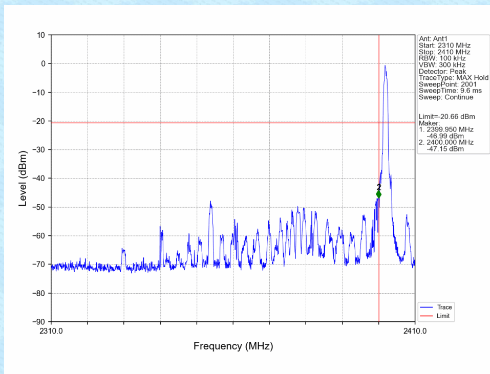
Pi/4DQPSK_2DH5_LCH_2402MHz_Ant1_NTNV
