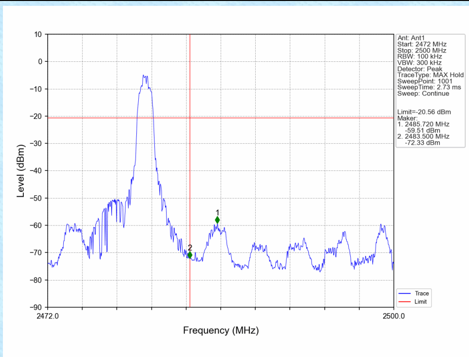
8DPSK_3DH5_HCH_2480MHz_Ant1_NTNV
