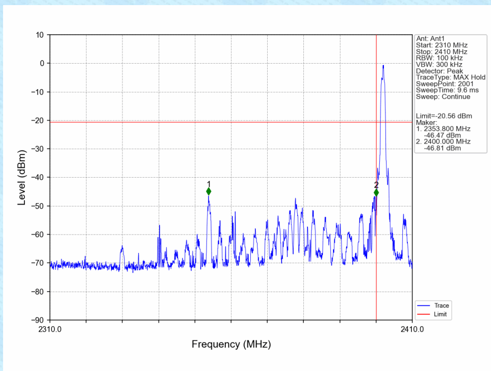
8DPSK_3DH5_LCH_2402MHz_Ant1_NTNV
