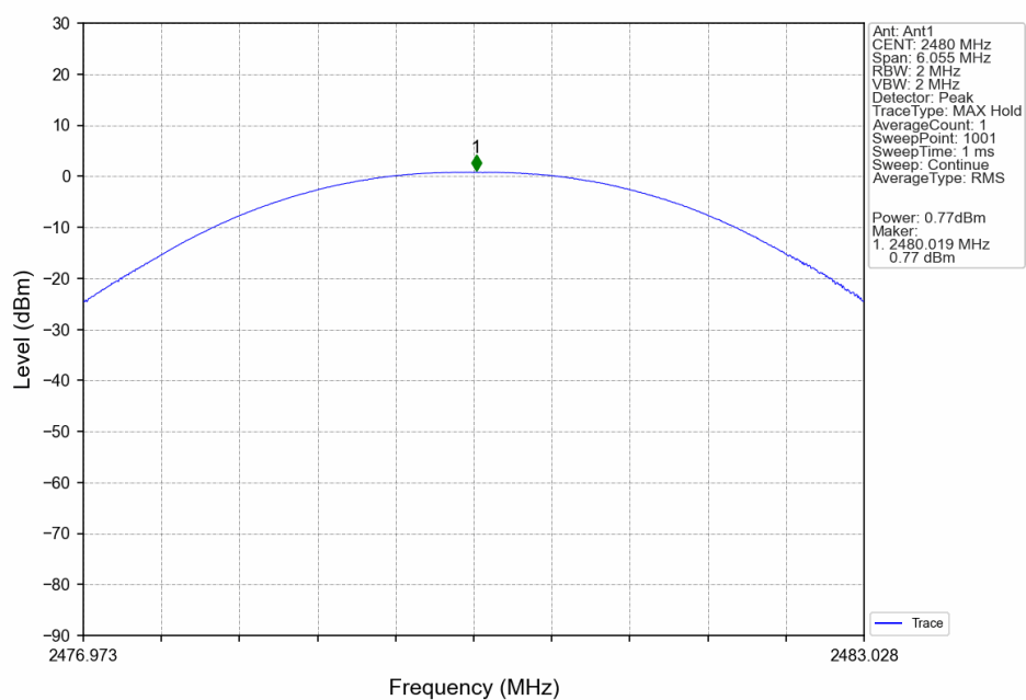
\pi /4QPSK_2DH5_HCH_2480MHz_Ant1_NTNV
