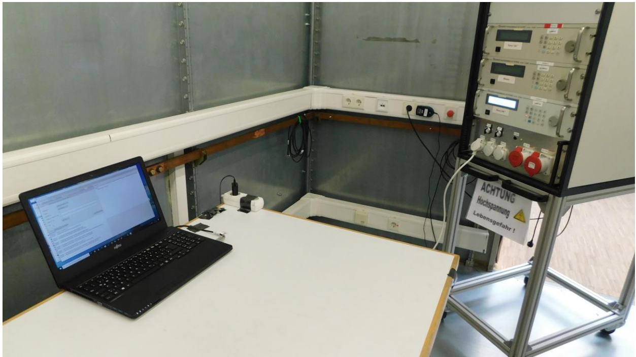
Picture 9: Test setup AC power line conducted emissions
