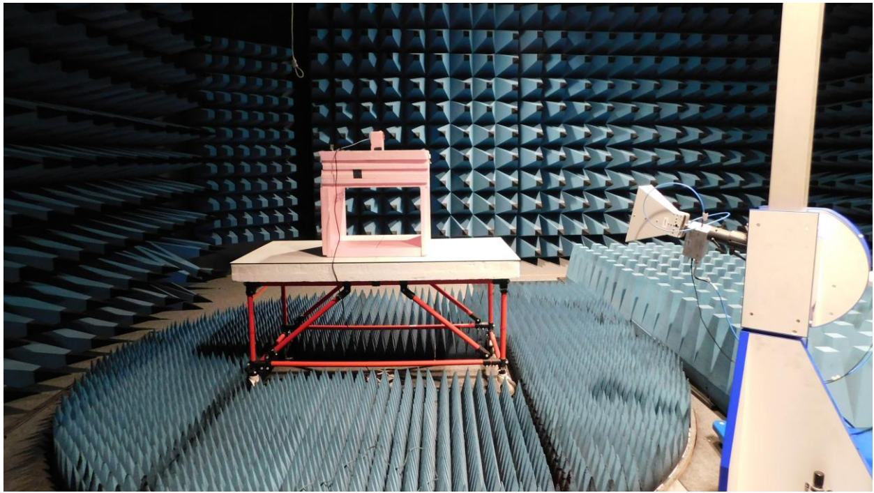
Picture 5: AC, radiated emission test 1 GHz – 18 GHz (front view)
