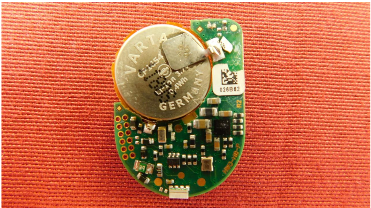
Picture 4: Radio module – back side
