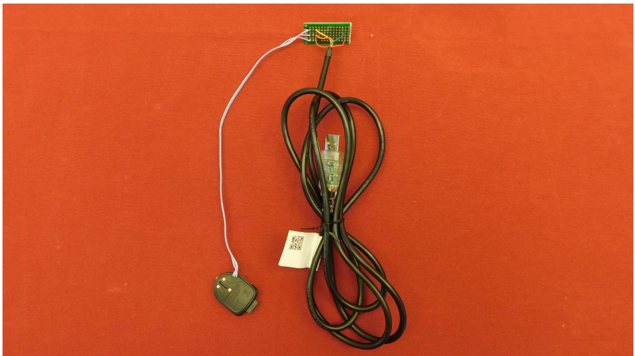
Picture 2: EUT without antenna cable – rear view
