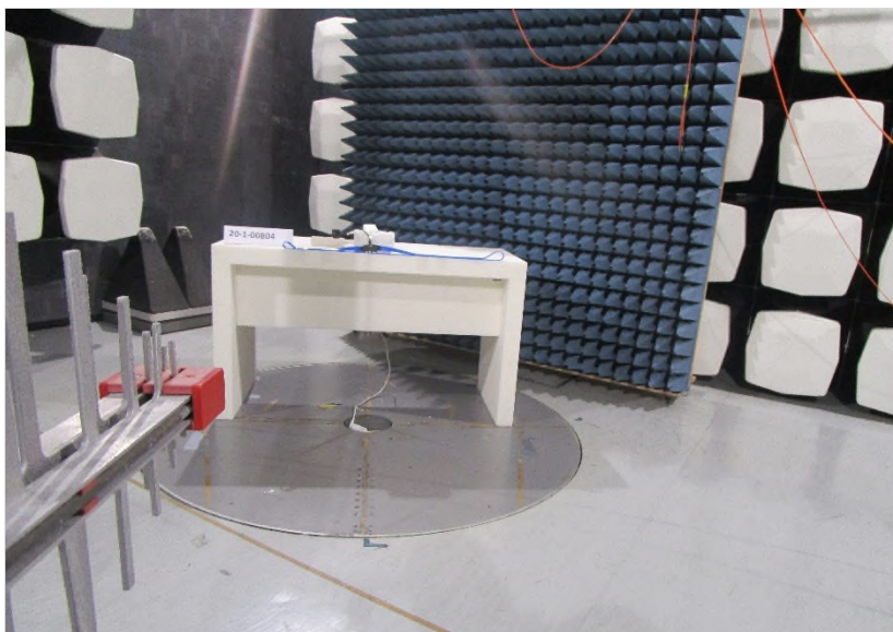
Photograph 2: EUT Test Setup in the anechoic chamber, overview
