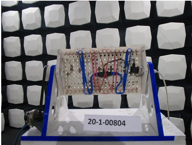
Photograph 5: EUT Test Setup in the fully anechoic chamber, close view
