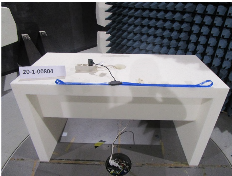
Photograph 3: EUT Test Setup in the anechoic chamber, close view
