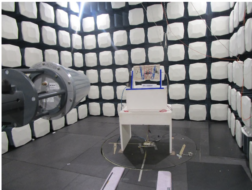
Photograph 4: EUT Test Setup in the fully anechoic chamber, overview
