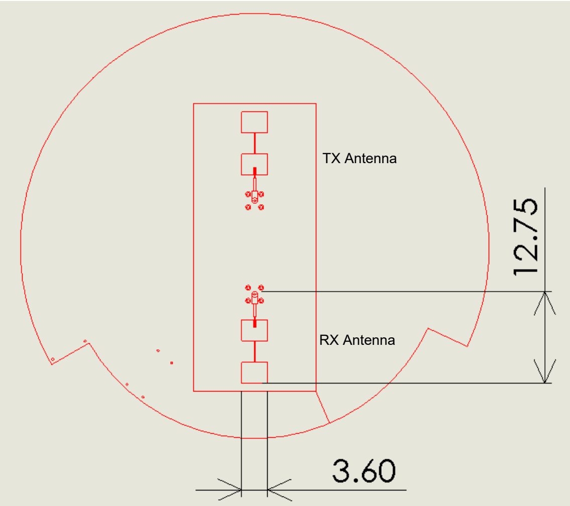
Dimensions (mm)
