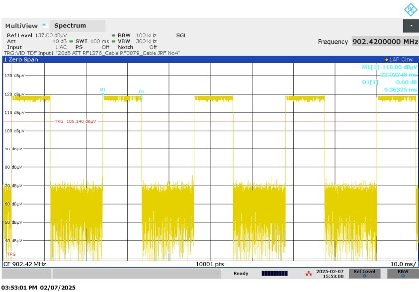
Figure 21: Maximum dwell time in 100ms window, Mode A (902.42MHz)
