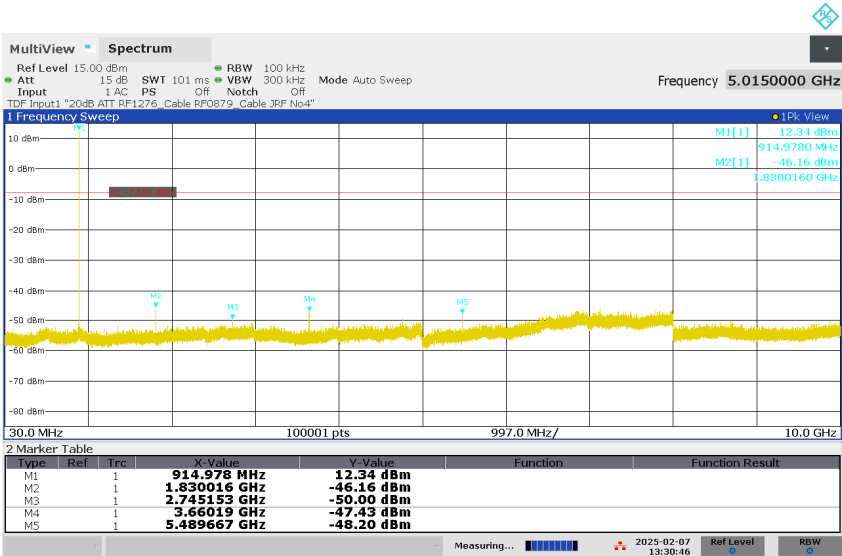
Figure 25: Conducted Spurious Emissions, 30MHz - 10GHz, Mode B (915.00MHz)
