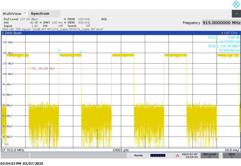
Figure 22: Maximum dwell time in 100ms window, Mode B (915.00MHz)
