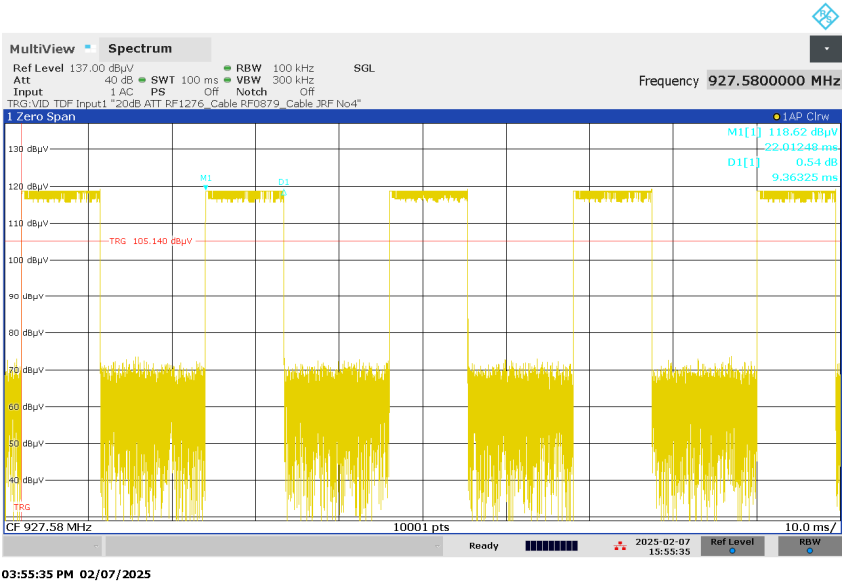
Figure 23: Maximum dwell time in 100ms window, Mode C (927.58MHz)
