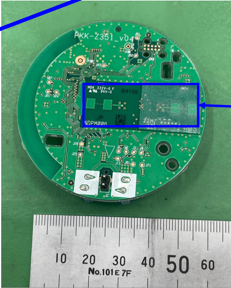
SubGHz Antenna
