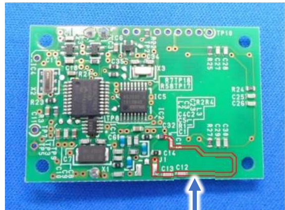
Pattern Antenna
