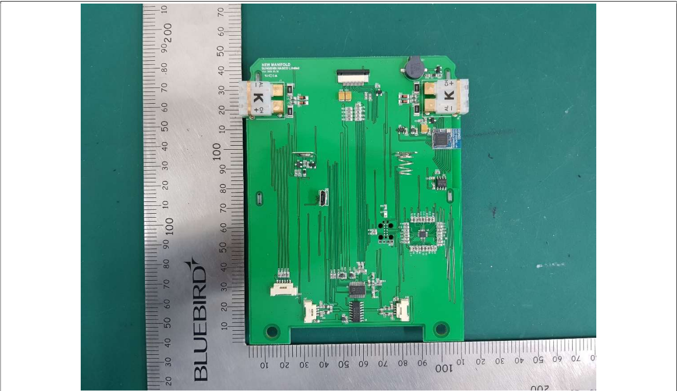
Main Board_Rear
