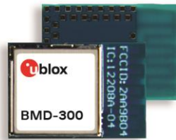
Figure 2: BMD-300 antenna as integrated
