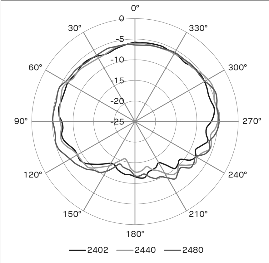
Figure 5 – Gain Y-Z
