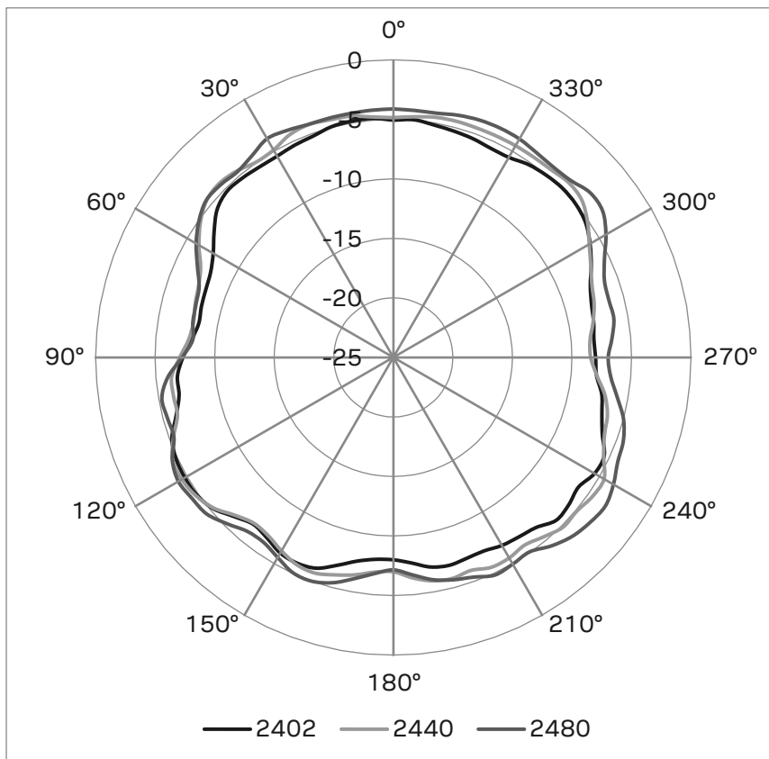
Figure 4 – Gain X-Z
