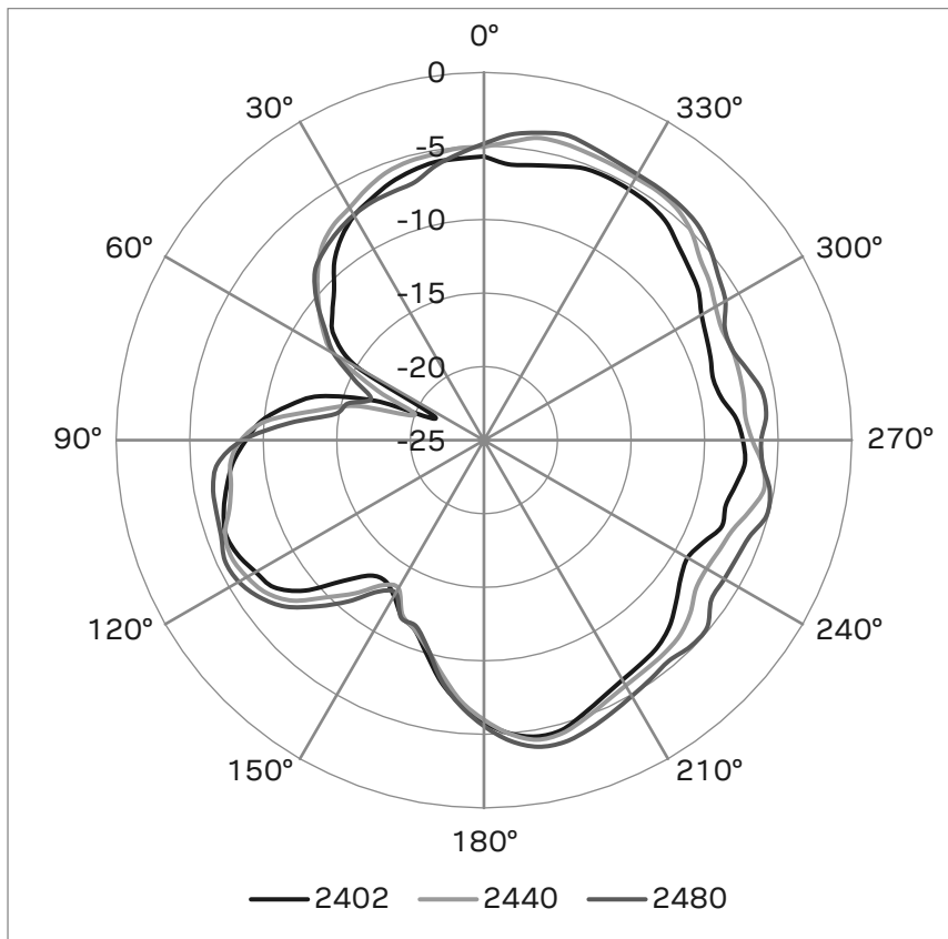
Figure 3 – Gain X-Y
