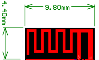
Figure 1: BMD-300 antenna layout
