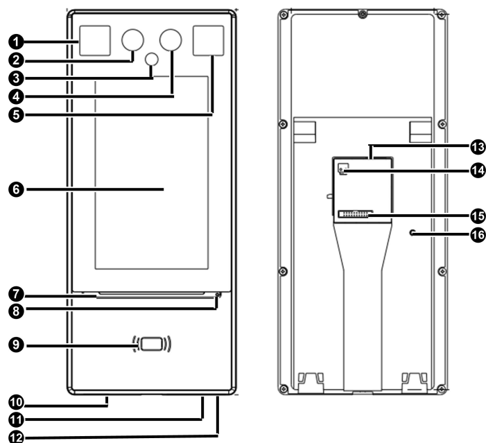
Figure 2-1 Device Structure
