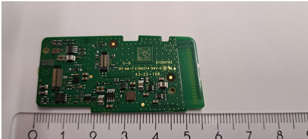
Figure 4 PCB system connector side
