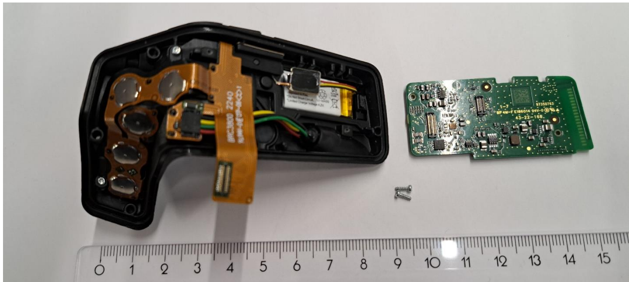
Figure 2 PCB removed
