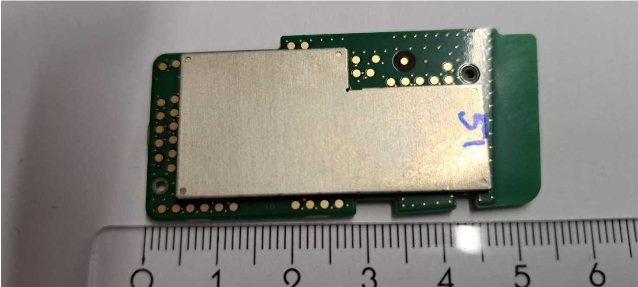
Figure 5 PCB shielded side
