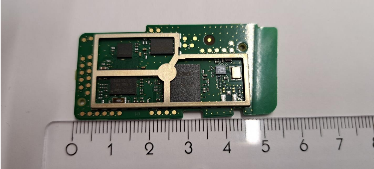
Figure 6 shield opened
