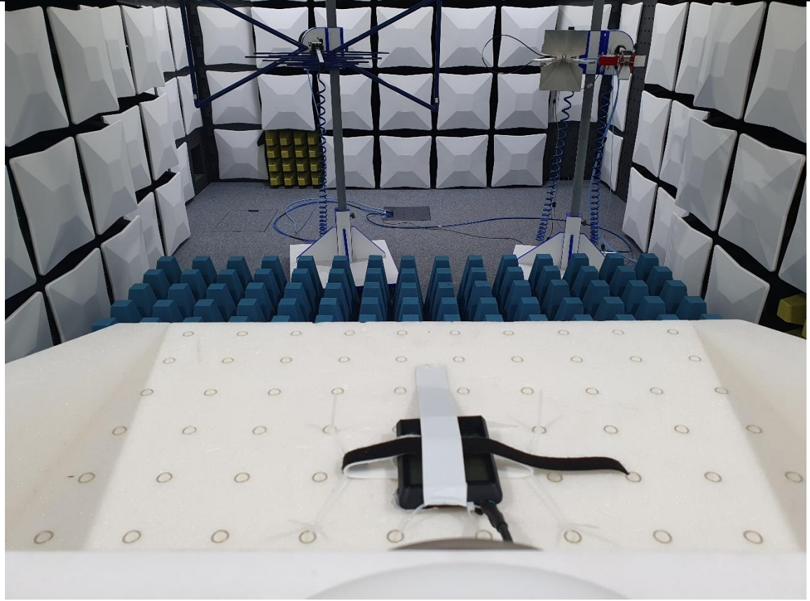
Test Setup: Radiated Measurements (1 GHz to 25 GHz) EUT side
