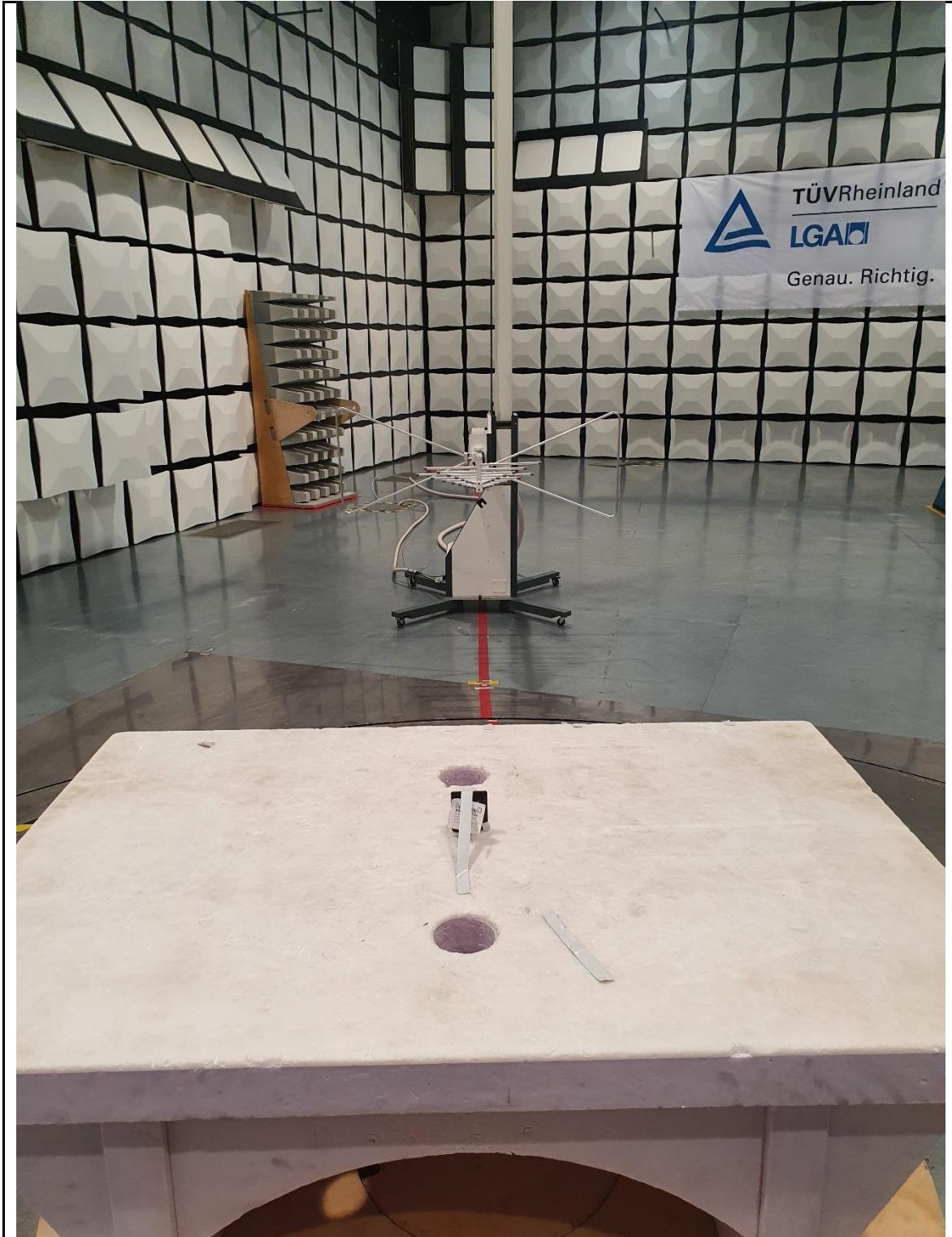
Test Setup: Radiated Measurements (30 MHz - 1 GHz) EUT side
