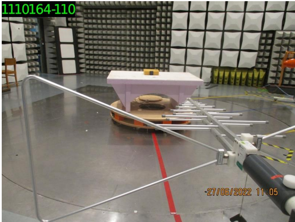
Test Setup: Radiated disturbance (30M - 1GHz) for 15B and ICES-003
