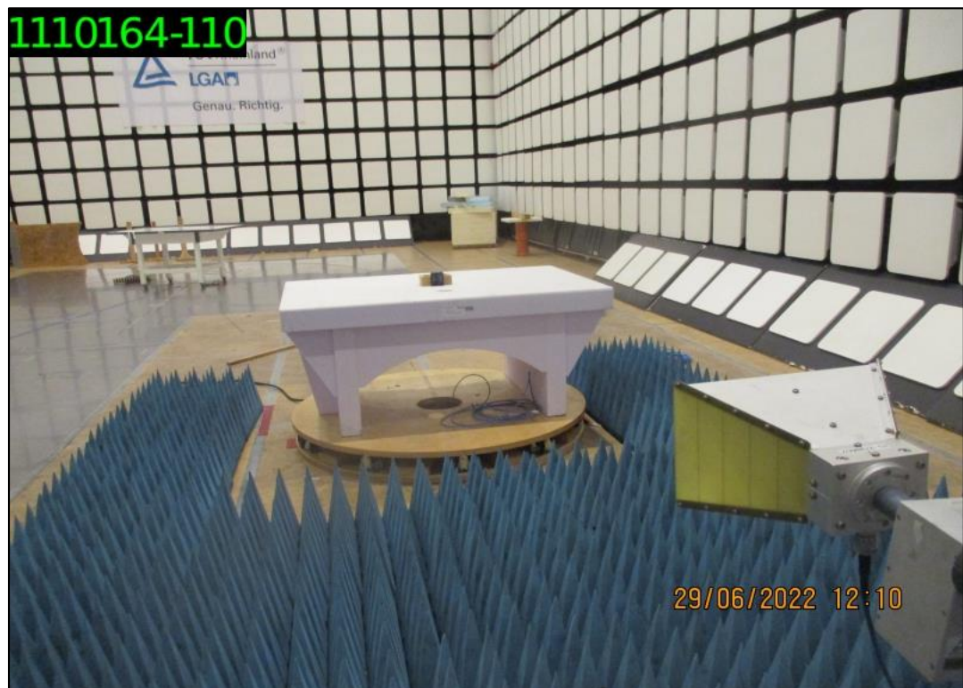
Test Setup: Radiated disturbance (> 1 GHz) for 15B and ICES-003
