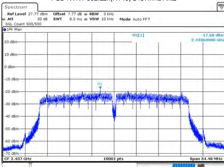
PSD NVNT 802.11n(HT40) 2437MHz Ant1
