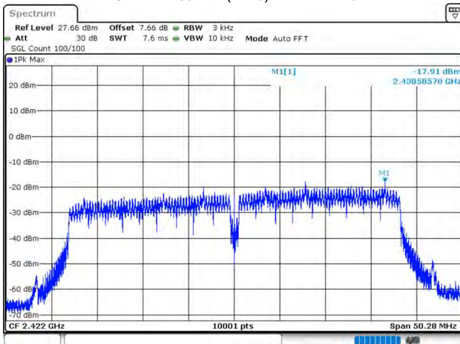
PSD NVNT 802.11n(HT40) 2422MHz Ant1
