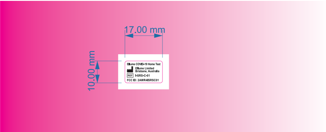
Wireless Analyser Gen II Compliance Decal Scale 1:1
