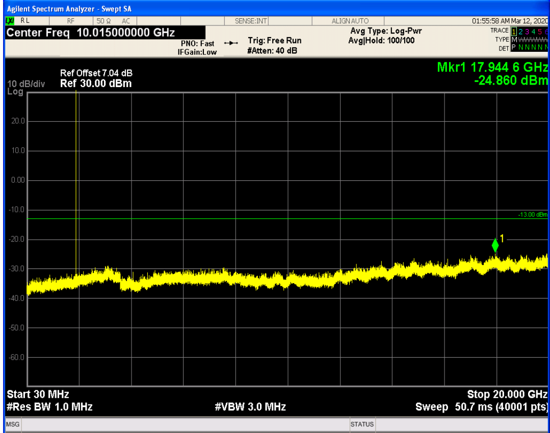
GPRS850 Channel=128
