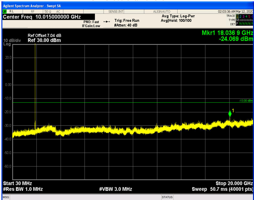
GPRS1900 Channel=661
