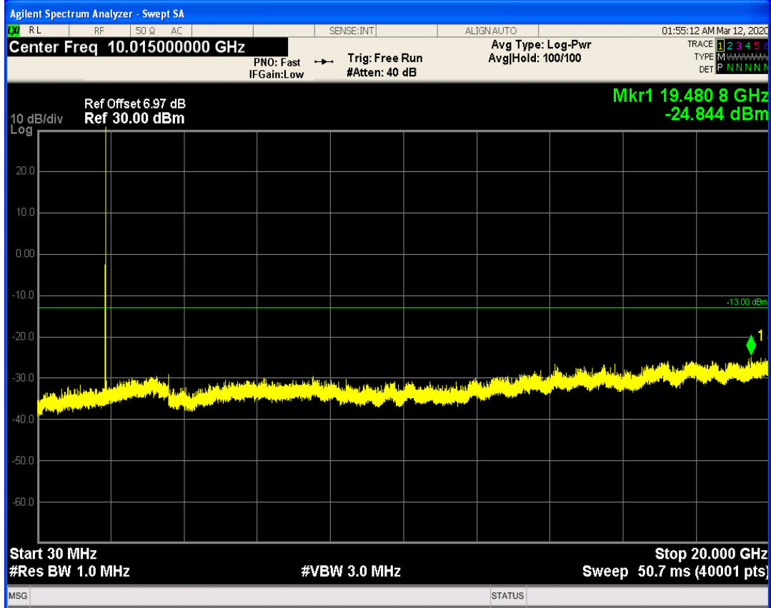
GSM1900 Channel=512
