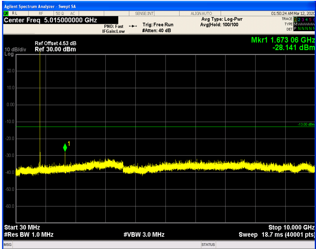
GSM850 Channel=251
