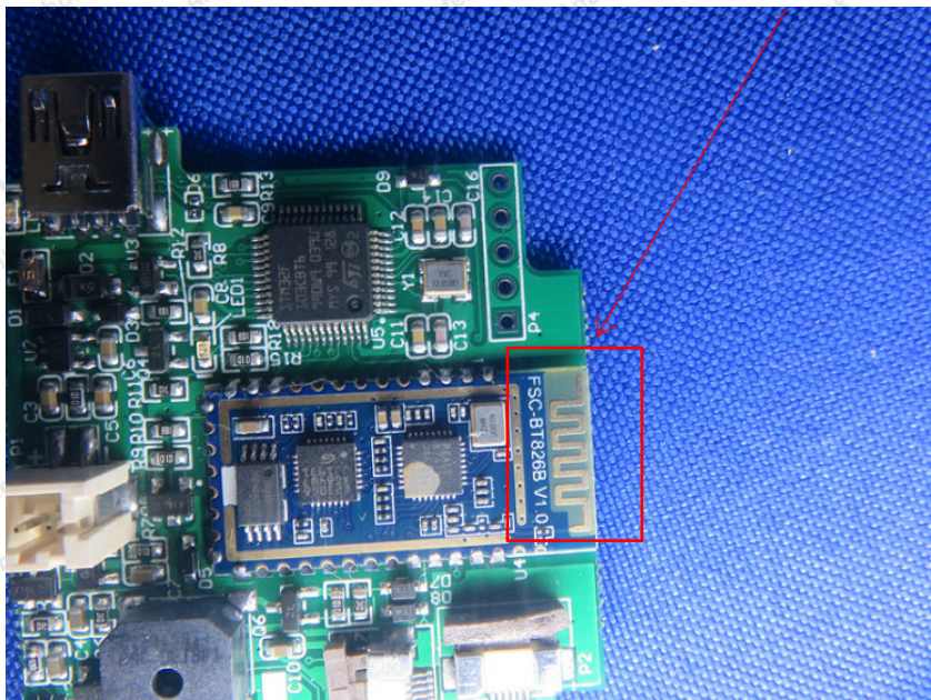
BT Antenna
