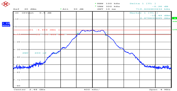
High 0.719MHz
