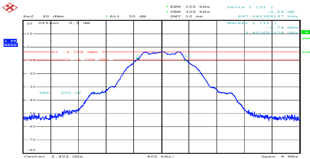
Low 0.697MHz
