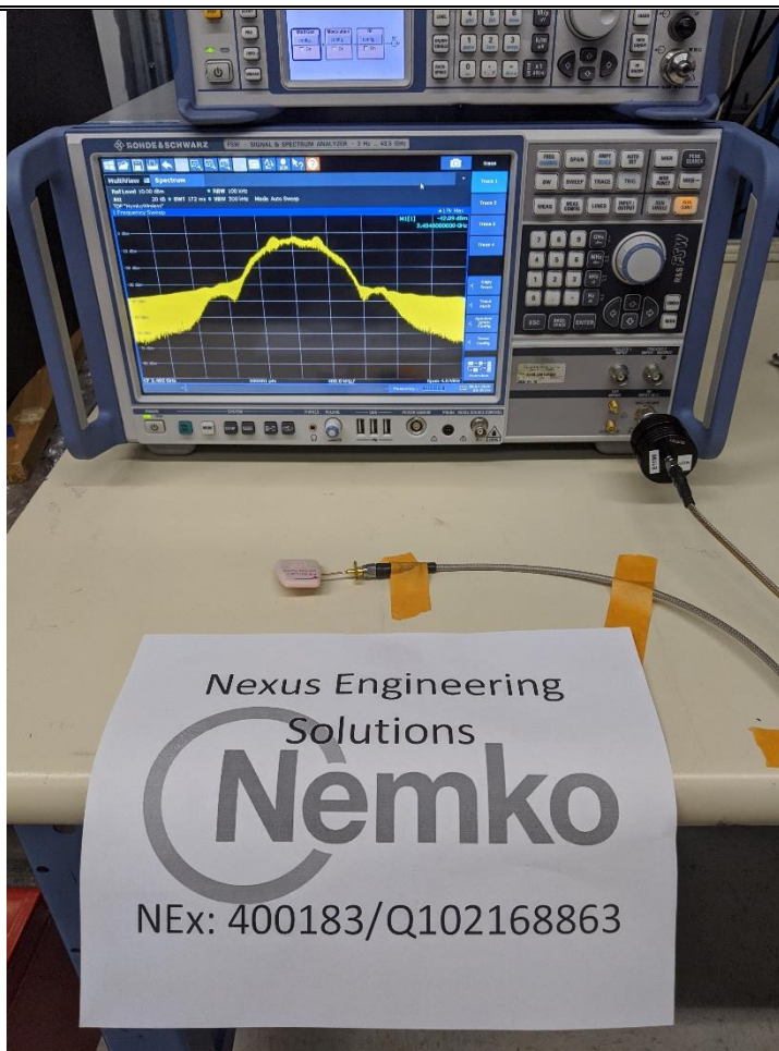
Figure 5 – Conducted antenna port test setup
