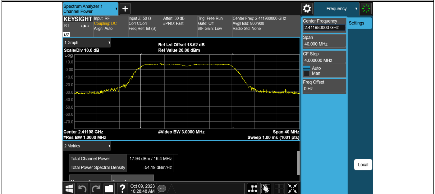
11G-Ant2-2412-PASS
