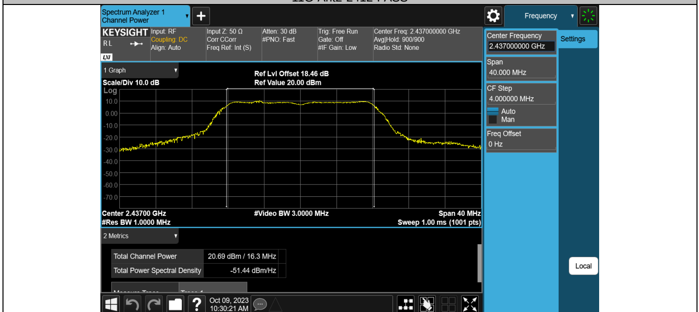
11G-Ant1-2437-PASS
