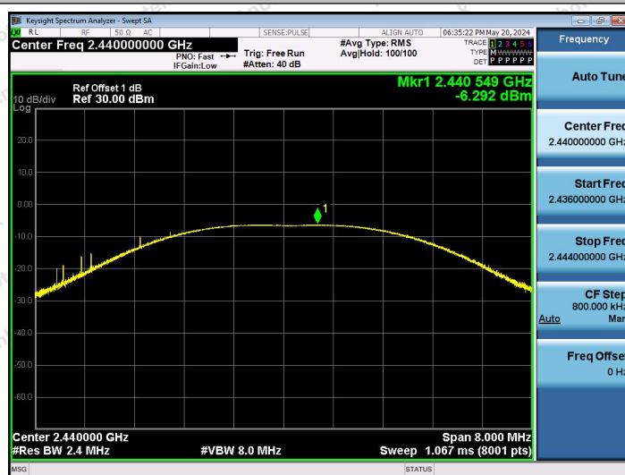
Zigbee-Ant1-2440-PASS
