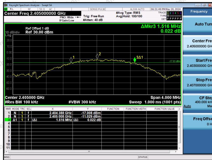
Zigbee-Ant1-2405-PASS
