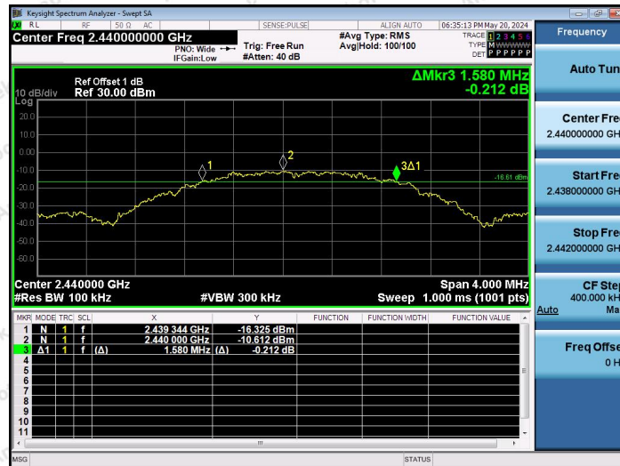
Zigbee-Ant1-2440-PASS
