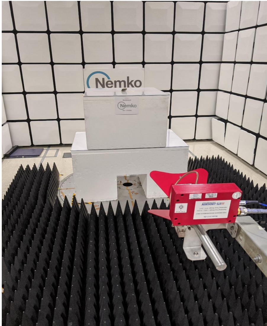
Figure 2 - Radiated emissions, 1 - 18 GHz, front view
