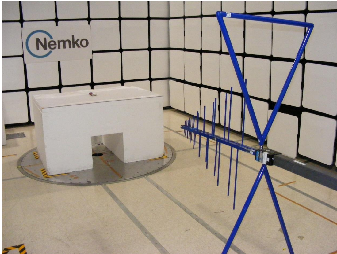
Figure 1 - Radiated emissions, 30 - 1000 MHz, front view
