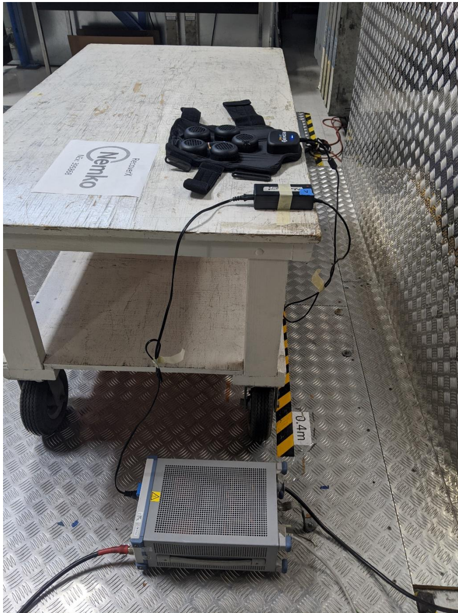
Figure 6 – AC conducted emissions, side view
