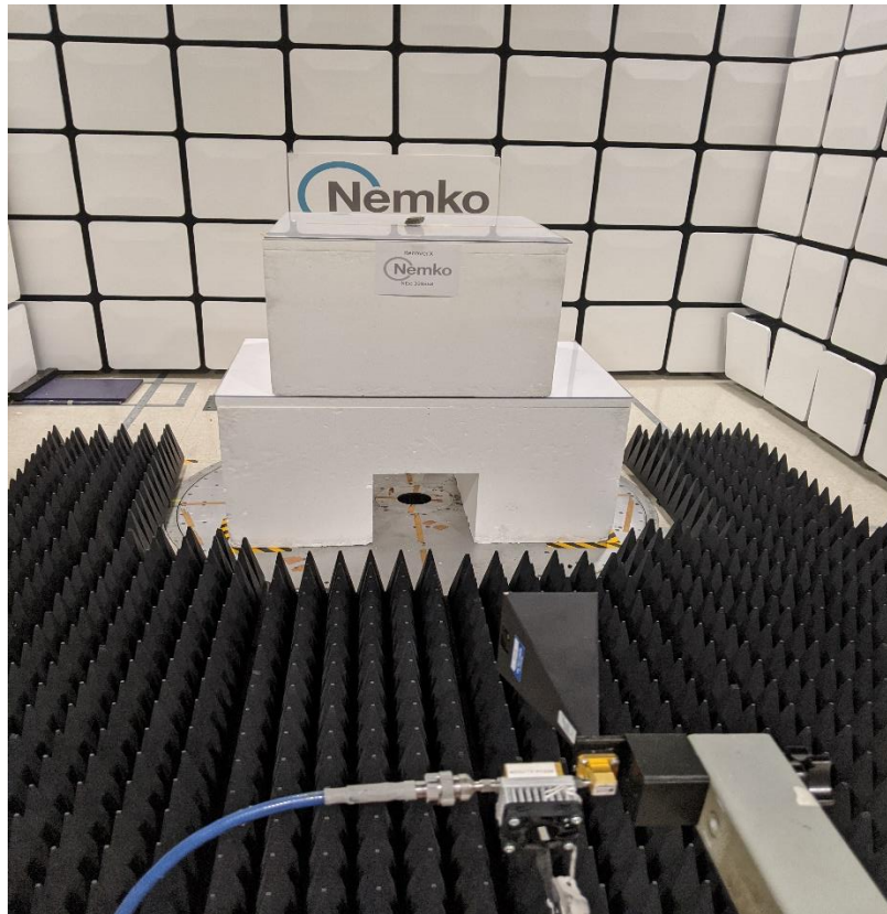
Figure 3 - Radiated emissions, 18 - 26 GHz, front view
